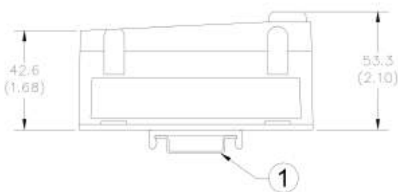
Figure 1: 990 Vibration Transmitter Dimensions (top view)
